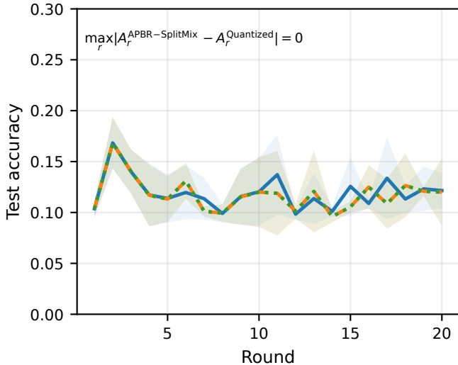
CIFAR-10
