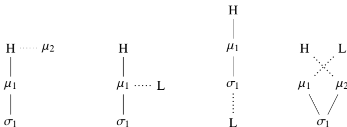
Figure 6: Invalid AR Expansion
