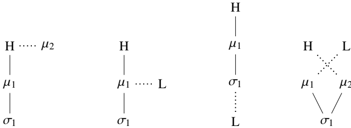
Figure 6: Invalid AR Expansions
