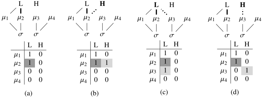
Figure 8: Three options to form new associations
