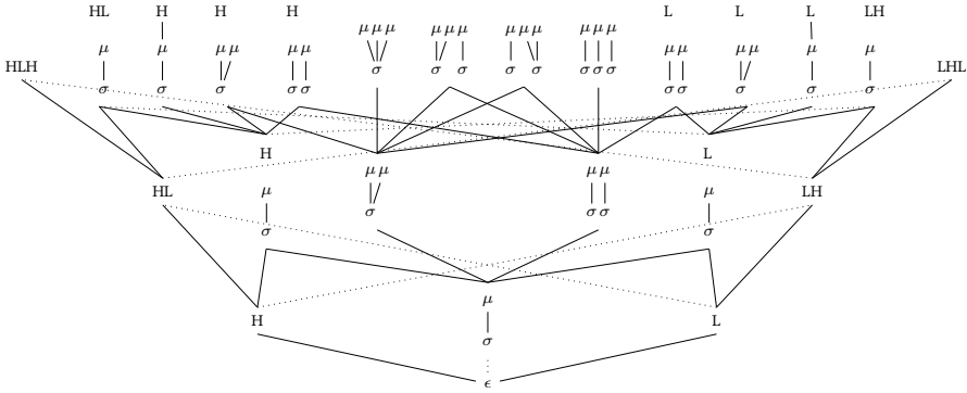
Figure 9: A partially-ordered hypothesis space over ARs
