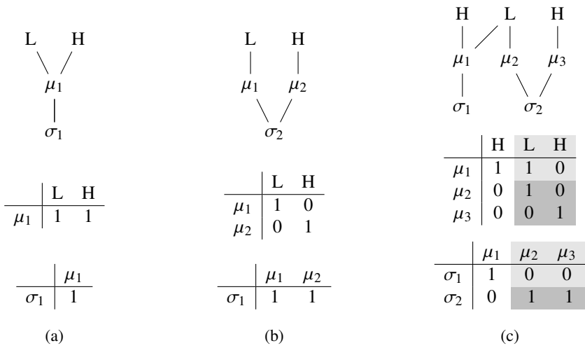
Figure 11: Light LH (11a), heavy LH (11b), and a superfactor of heavy LH (11c)
