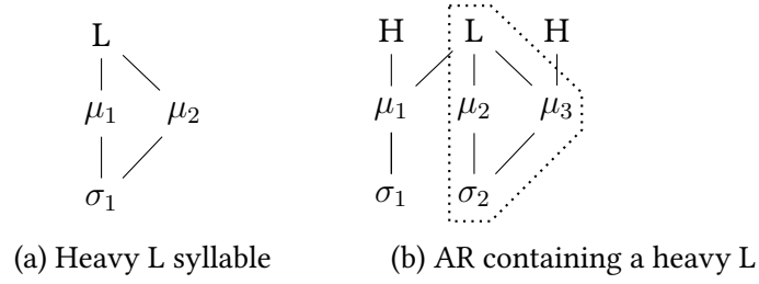
Figure 3.3: A heavy L-toned syllable and a structure in which it is contained
