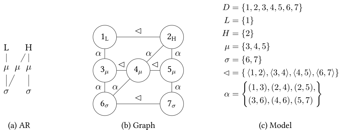
Figure 3.2: Three representations of a disyllabic LH.H
