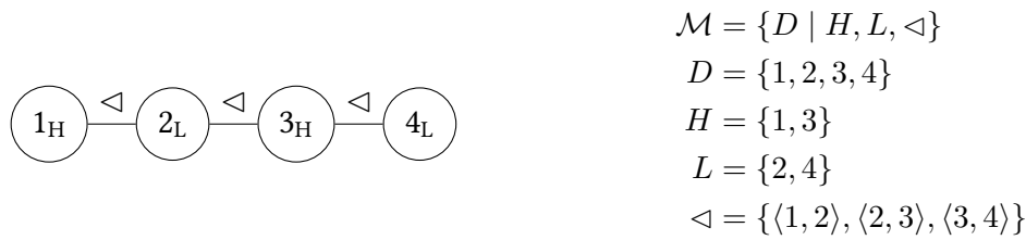
Figure 3.1: String model for HLHL over \Sigma = \{H, L\} .
