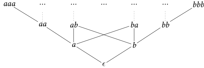
Figure 3.4: Strings over \Sigma = \{a, b\} ordered by the containment relation (non-exhaustive)
