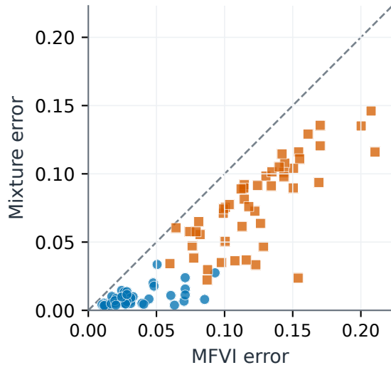
(b) Covariance error
