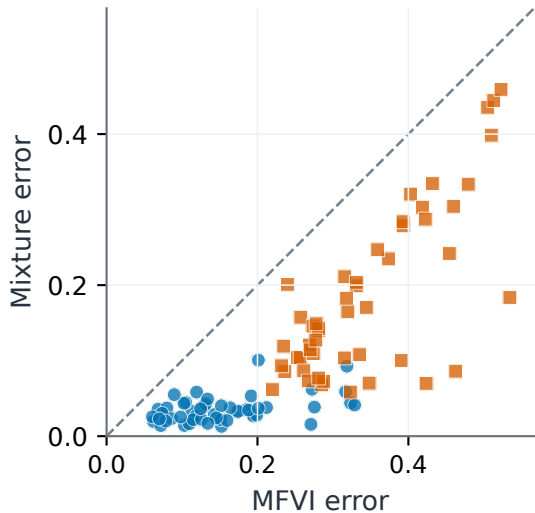
(a) Joint-support error (TV)
