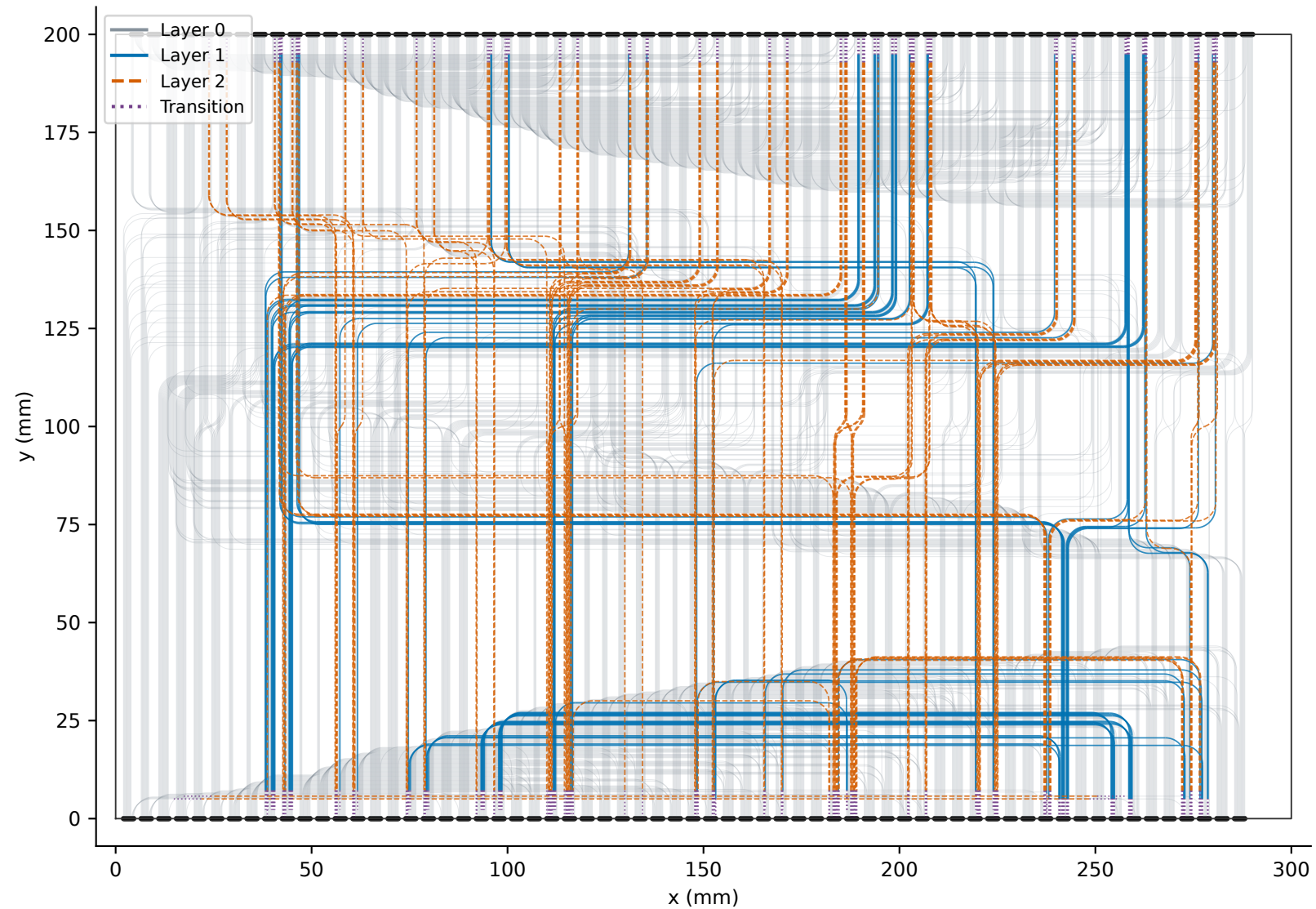
All 1024 routes: XY projection; PMTs and endpoints on board edges
