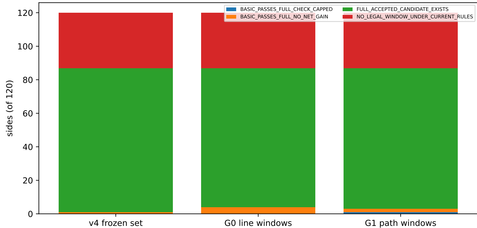
frozen 60-pair / 120-side diagnostic: outcome per generation domain
