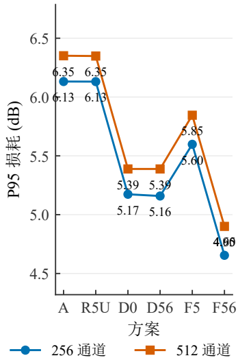
(b) P95 损耗
