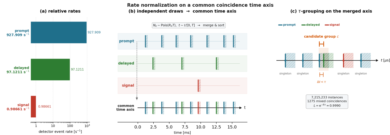
Figure 4: Rate normalization on a common coincidence time axis. (a) Full-band detector event rates (928, 97.1, and 0.987 s -1 ). (b) Independent Poisson draws of the three streams are merged and time-ordered; color marks stream identity and hatched bands mark each event’s temporal footprint. (c) Events with \Delta t \leq \tau = 1 \mu\text{s} form one candidate group; the box gives the reference-exposure accidental bookkeeping. Tick positions are schematic.
