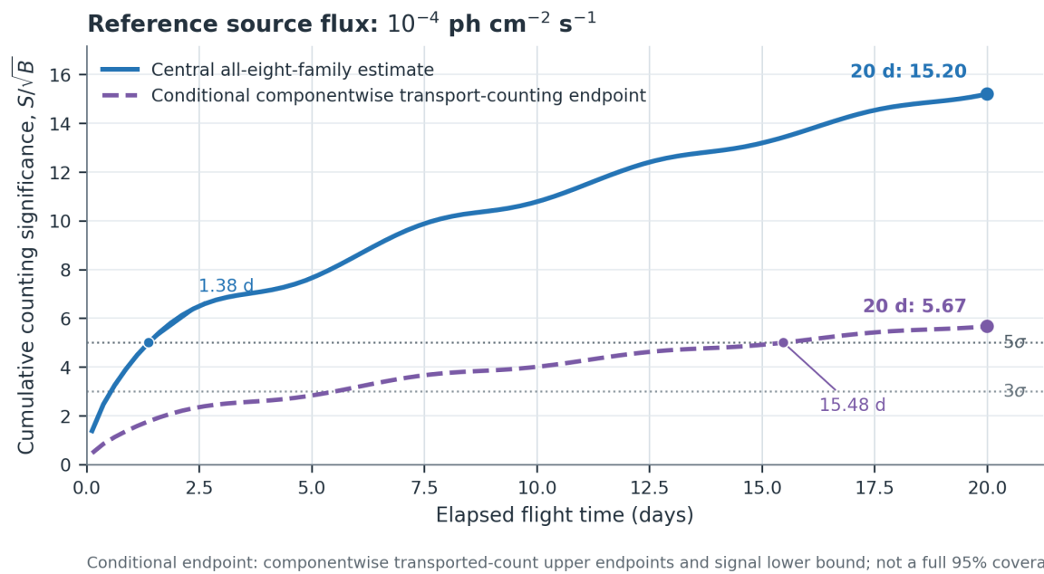
Figure 10: Cumulative counting significance of the final graded-shield geometry for a continuously observed 10^{-4} \text{ ph cm}^{-2} \text{ s}^{-1} point source along the 20 d reference trajectory. The solid curve uses the central selected rates. The dashed curve uses the upper exact 95% counting endpoints for every background component and the lower exact 95% signal-acceptance endpoint. Their componentwise combination is conditional, not a joint 95% interval. The curves reach 5\sigma at 1.38 and 15.48 d, respectively, and end at 15.20 and 5.67.
