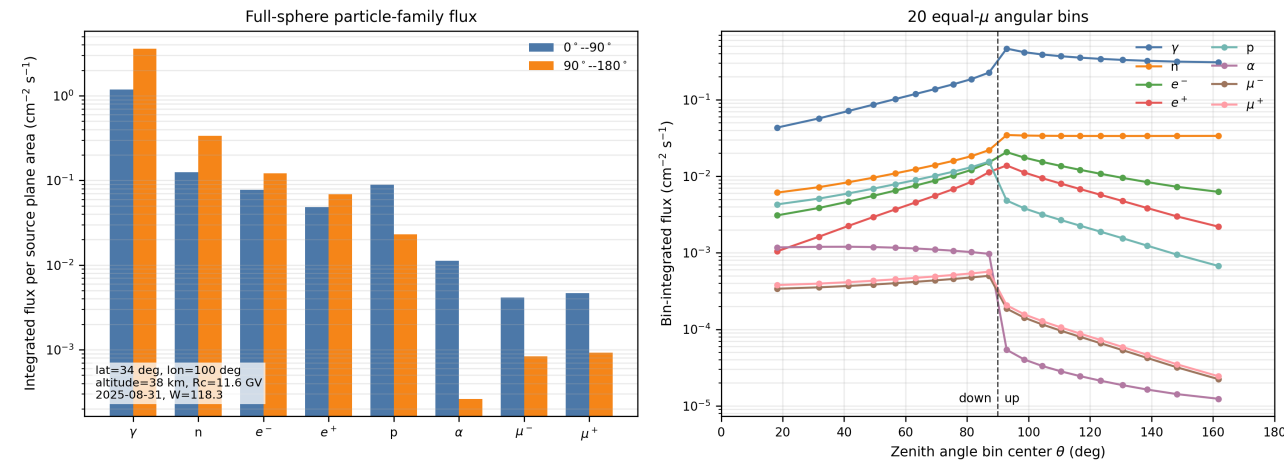
Figure 3: EXPACS/PARMA full-sphere atmospheric flux field used to generate the prompt and activation-production transport inputs. Left: energy- and solid-angle-integrated fluxes for the eight transported particle families, separated into down-going and up-going hemispheres. Right: bin-integrated flux in the 20 equal- \mu differential zenith bins used by the MEGALib far-field source. The plot is generated from the source-definition inputs for latitude 34^\circ , longitude 100^\circ , altitude 38 km, R_c = 11.6 GV, and W = 118.3 .
