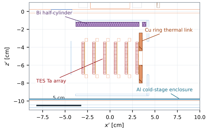
c SG3 Bi/TES transverse detail
