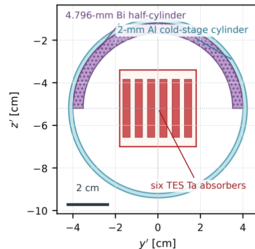
c SG3 Bi/TES transverse detail
