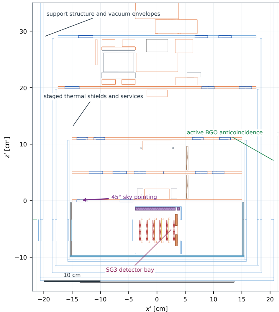
a Complete SG3 detector-cryostat mass model
