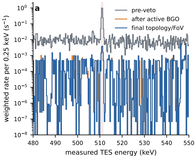
SH3 response spectrum
