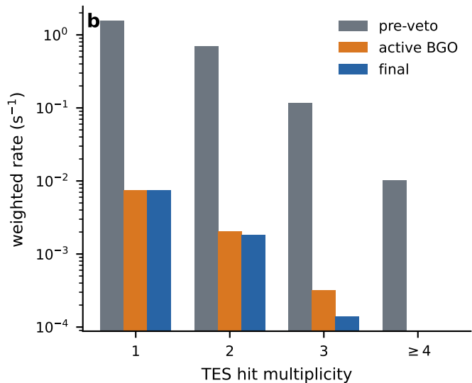
510.58--511.42 keV window
