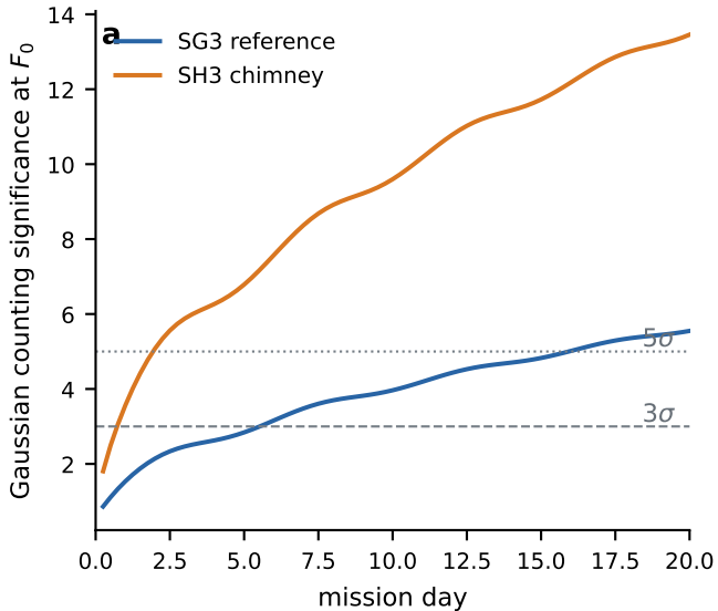
Cumulative significance
