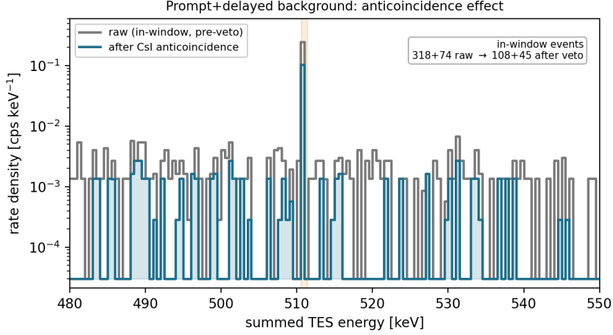
Figure 6: Effect of the CsI anticoincidence gate on the prompt+delayed background spectrum (in-window pre-veto vs after the shield gate). Shape-diagnostic re-derivation on the surviving Mass_model_511 catalogues.
