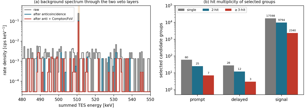
Figure 7: (a) Background spectrum through the two veto layers (raw; after anticoincidence; after anticoincidence+Compton/FoV). (b) Hit multiplicity of the selected candidate groups per stream. Shape-diagnostic re-derivation on the surviving Mass_model_511 catalogues; absolute rates are authoritative in Table 2.
