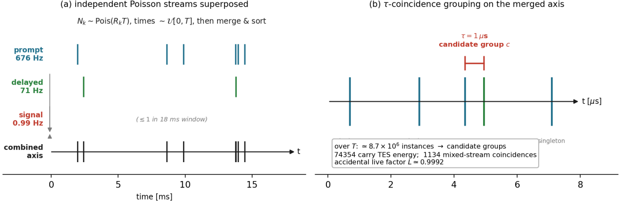
Figure 4: Schematic of the rate normalization. (a) The prompt, delayed, and focused-signal streams are drawn as independent homogeneous-Poisson processes at their full-band coincidence-axis rates and merged, time-ordered, onto one axis; (b) events within \tau = 1 \mu\text{s} form one candidate group, with the accidental-coincidence bookkeeping over the reference exposure annotated (baseline values). Tick positions in (a) are an illustrative Poisson realization.
