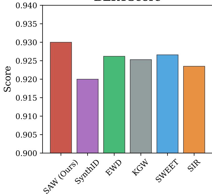
BERTScore
