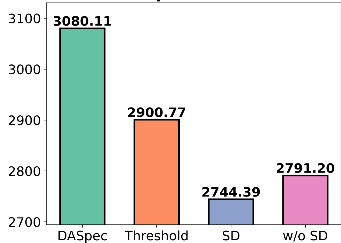
Specbench
