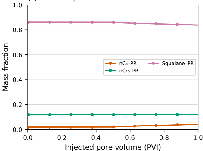
(c) Four-component PR: HC-normalized
