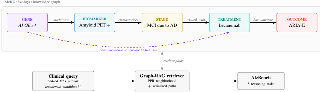
Figure 1: Overview of ALZGRAPH. ALZKKG links five clinical layers (gene, biomarker, stage, treatment, outcome) with typed relations; a representative reasoning path is highlighted. Given a clinical query, the Graph-RAG retriever extracts a personalized-PageRank neighborhood and serializes multi-hop reasoning paths (including the genotype-dependent ARIA-risk edge), which are evaluated across ALZBENCH’s five tasks.
