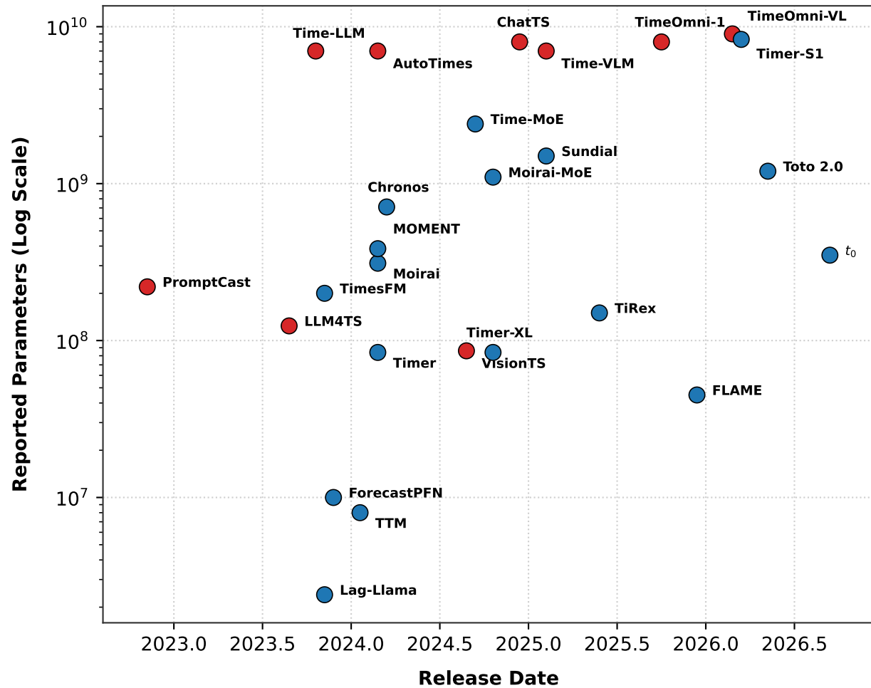
(a) Model Parameter Count vs. Release Date
