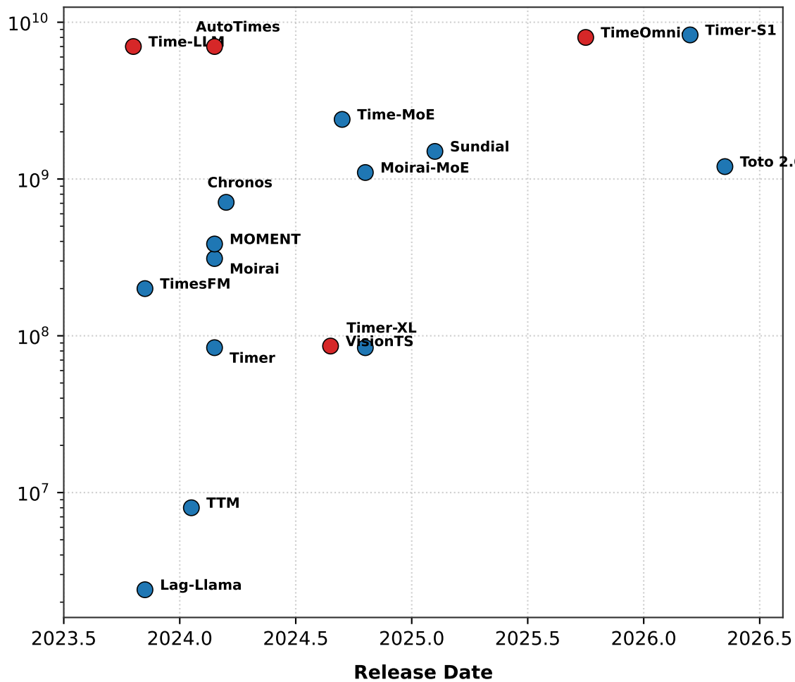
(a) Model Parameter Count vs. Release Date
