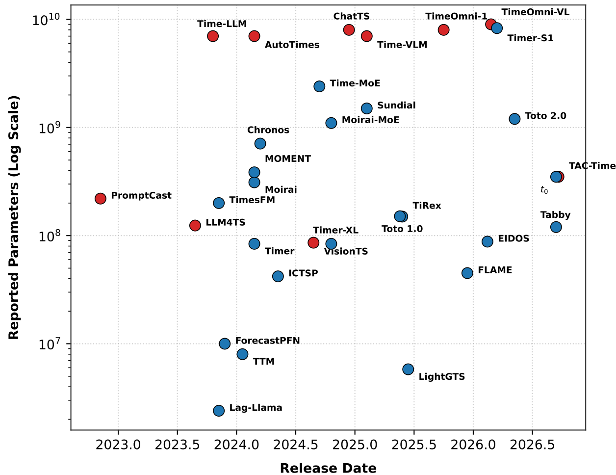
(a) Model Parameter Count vs. Release Date
