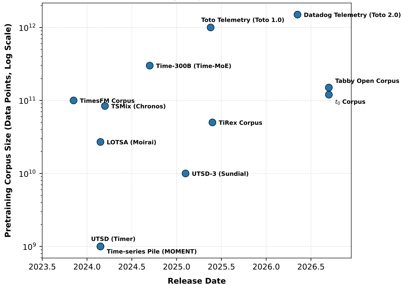
(b) Stated Pretraining Corpus Size vs. Release Date
