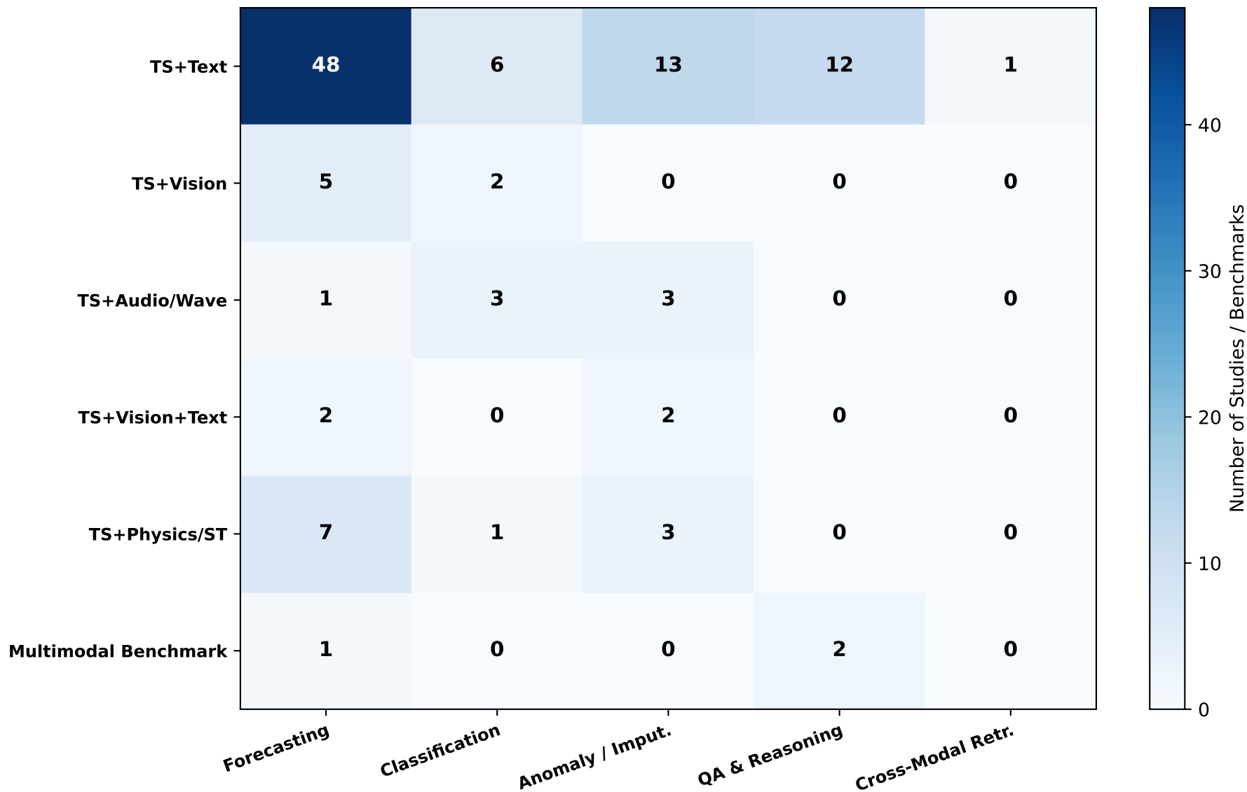
Cross-Distribution: Modality Pairings vs. Downstream Tasks (N=77)
