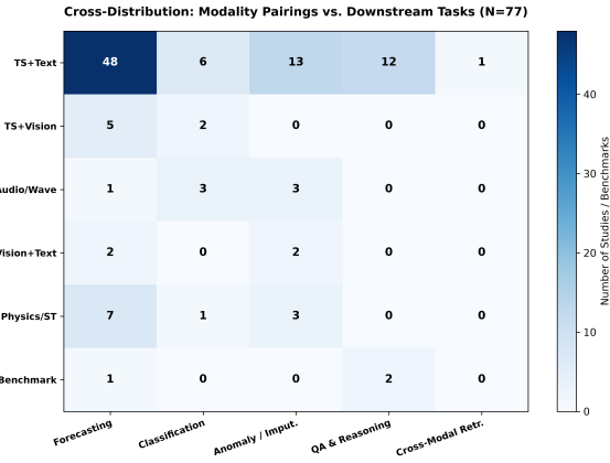
Fig. 11. Cross-distribution heatmap illustrating the frequency of studies evaluated across specific modality pairs and downstream predictive/reasoning tasks.
