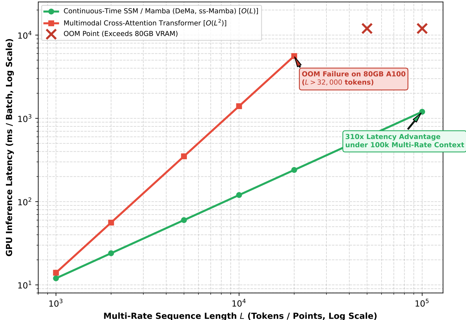
(b) Long-Context Inference Latency vs. Sequence Length ( L )
