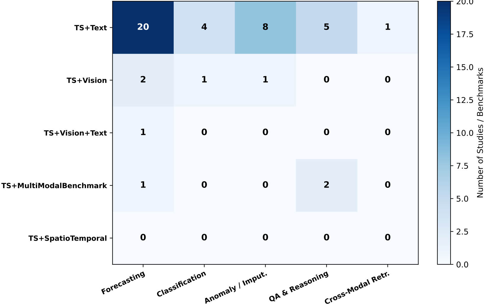
Cross-Distribution: Modality Pairings vs. Downstream Tasks
