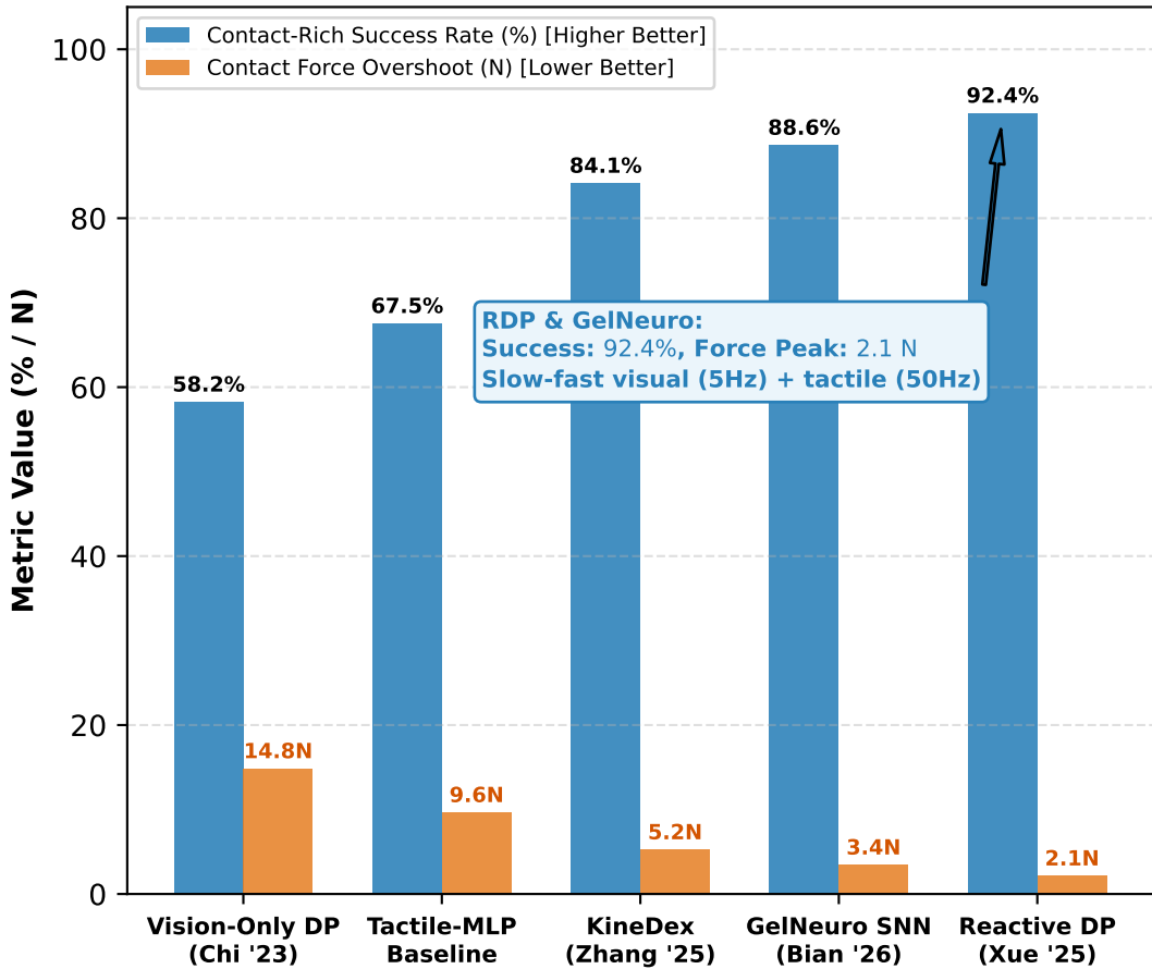
(a) Visuo-tactile Diffusion & Neuromorphic Skin: Contact-Rich Success vs Force Overshoot
