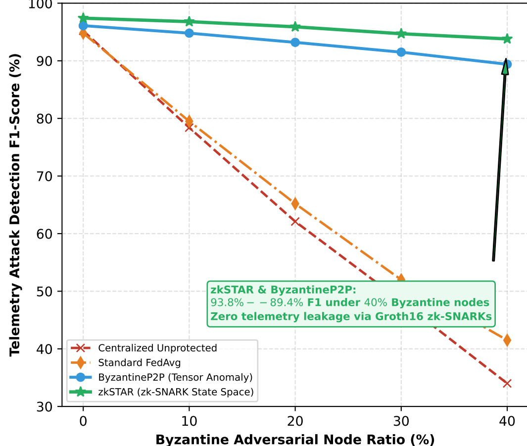
(c) Decentralized Smart Grid Telemetry: Byzantine Resilience & Zero-Knowledge Proofs
