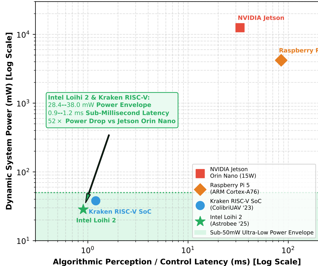
(c) Edge Neuromorphic Silicon Co-Design: Sub-50mW Ultra-Fast Closed-Loop Control
