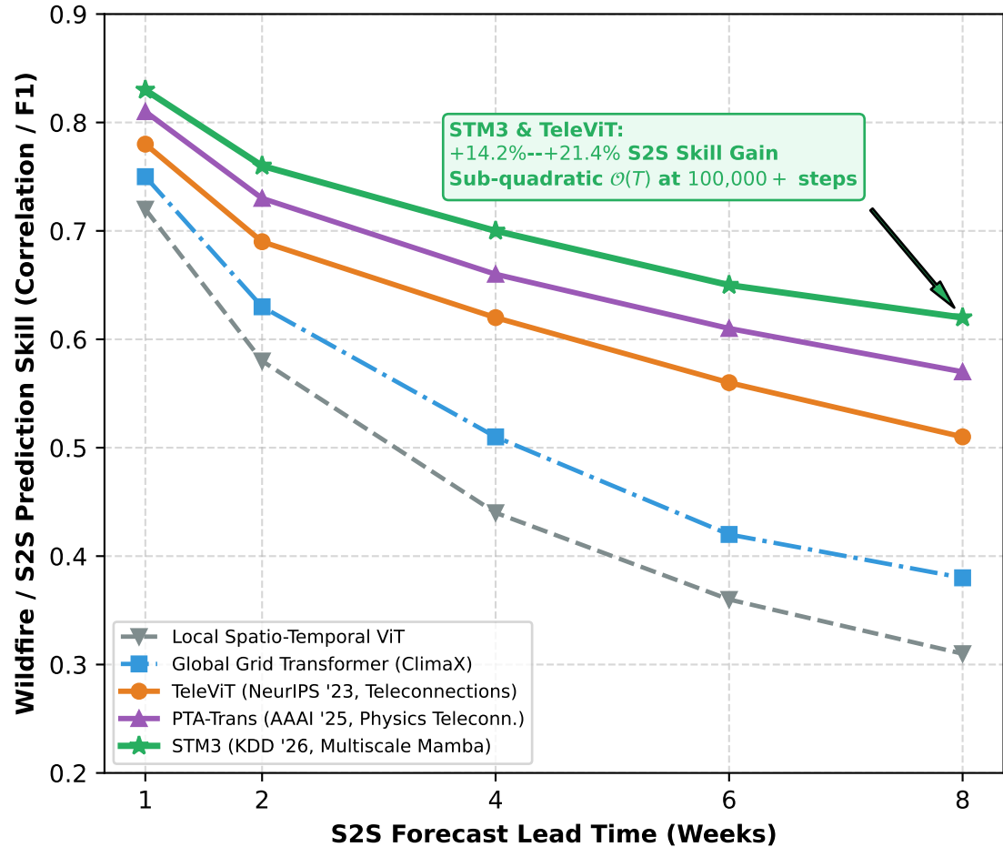
(a) Multi-Decadal Earth Teleconnections: Prediction Skill vs S2S Lead Time
