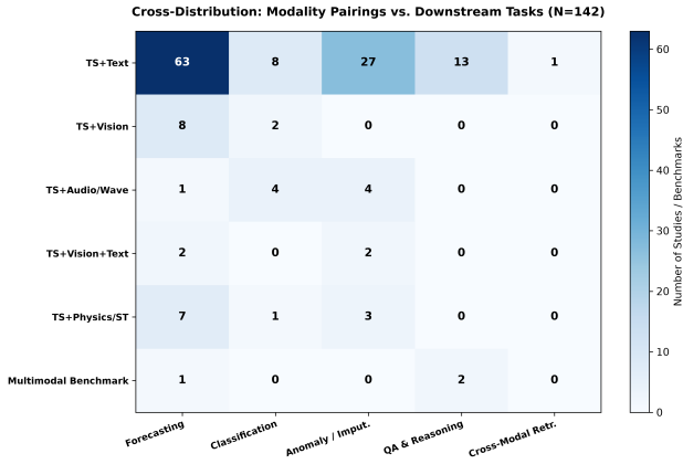
Fig. 19. Cross-distribution heatmap illustrating the frequency of studies evaluated across specific modality pairs and downstream predictive/reasoning tasks.
