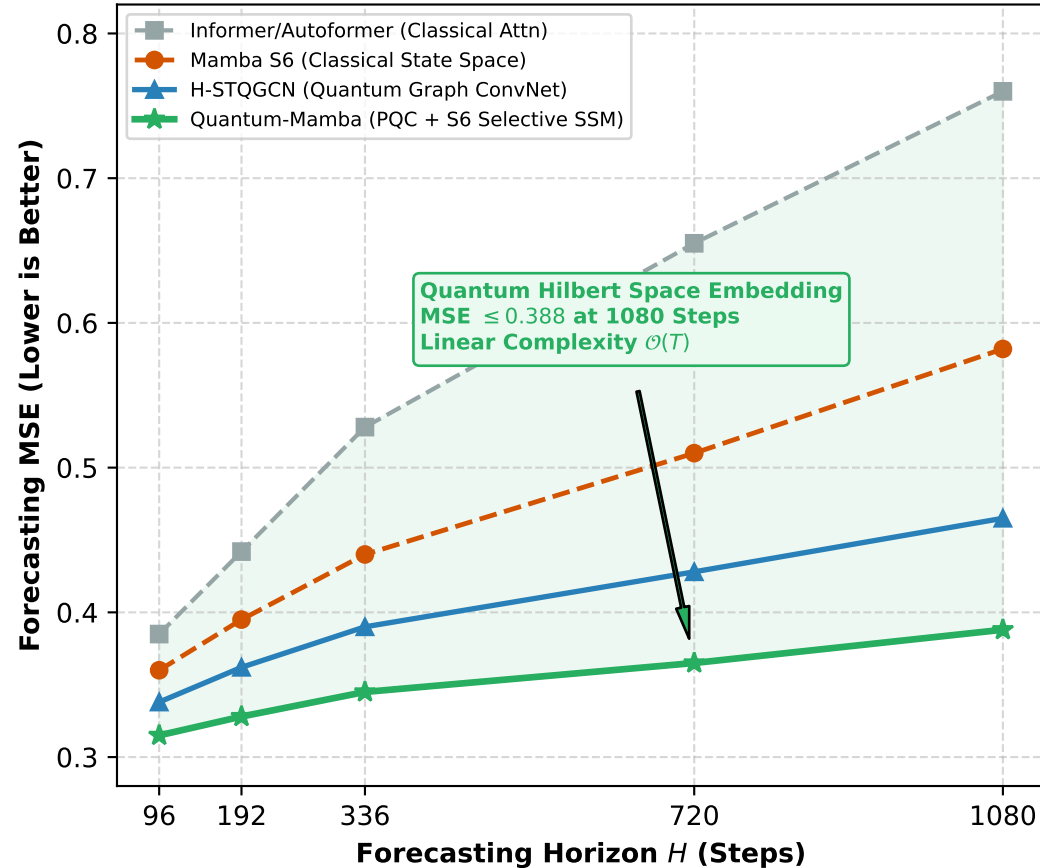
(b) Long-Term Spatio-Temporal Forecasting in Quantum-Classical State Spaces
