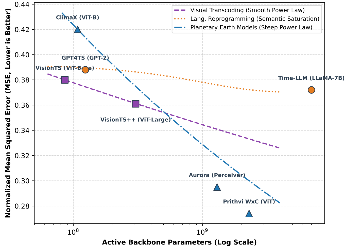
(a) Parameter Scaling Laws Across Multimodal Paradigms
