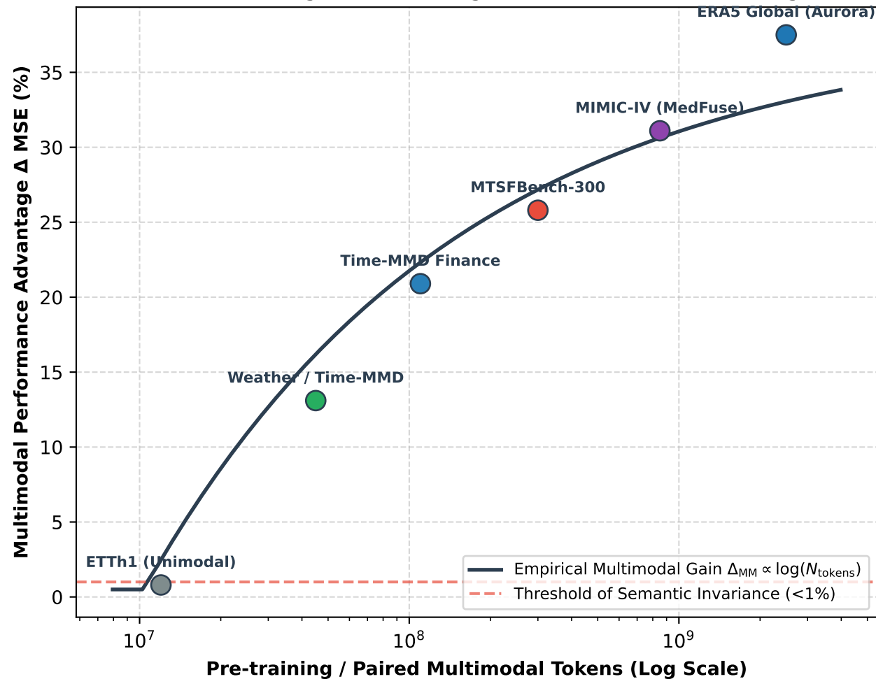
(b) Pre-training Token Scaling & Semantic Gain Advantage
