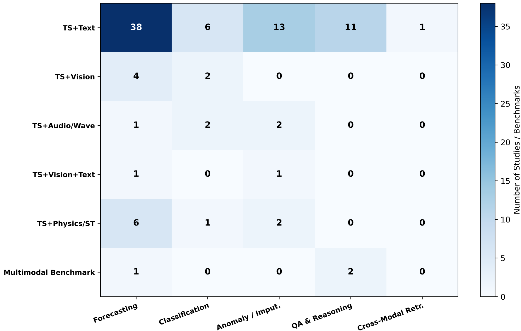
Cross-Distribution: Modality Pairings vs. Downstream Tasks (N=63)
