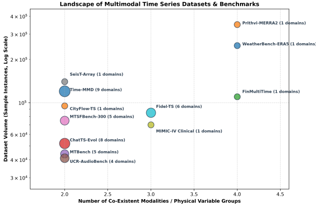
Fig. 9. Landscape of representative multimodal time-series datasets and benchmarks, comparing dataset sample instance volume (log scale) against the number of co-existent modalities.
