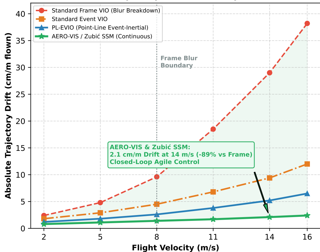
(a) Autonomous UAV Flight under Turbulence: Trajectory Drift vs Velocity
