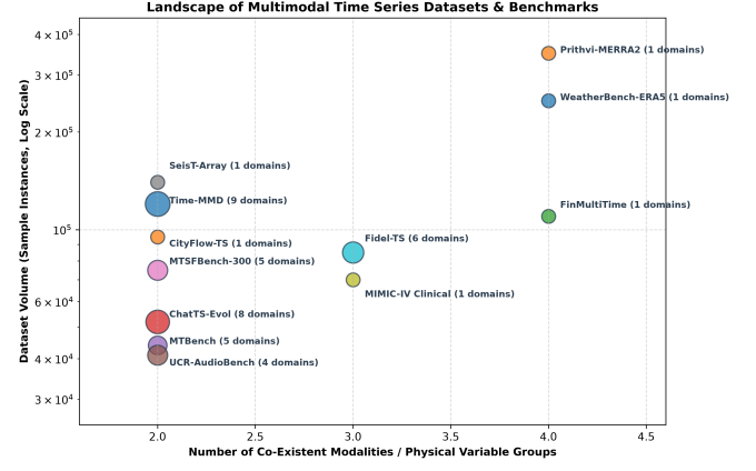
Fig. 17. Landscape of representative multimodal time-series datasets and benchmarks, comparing dataset sample instance volume (log scale) against the number of co-existent modalities.
