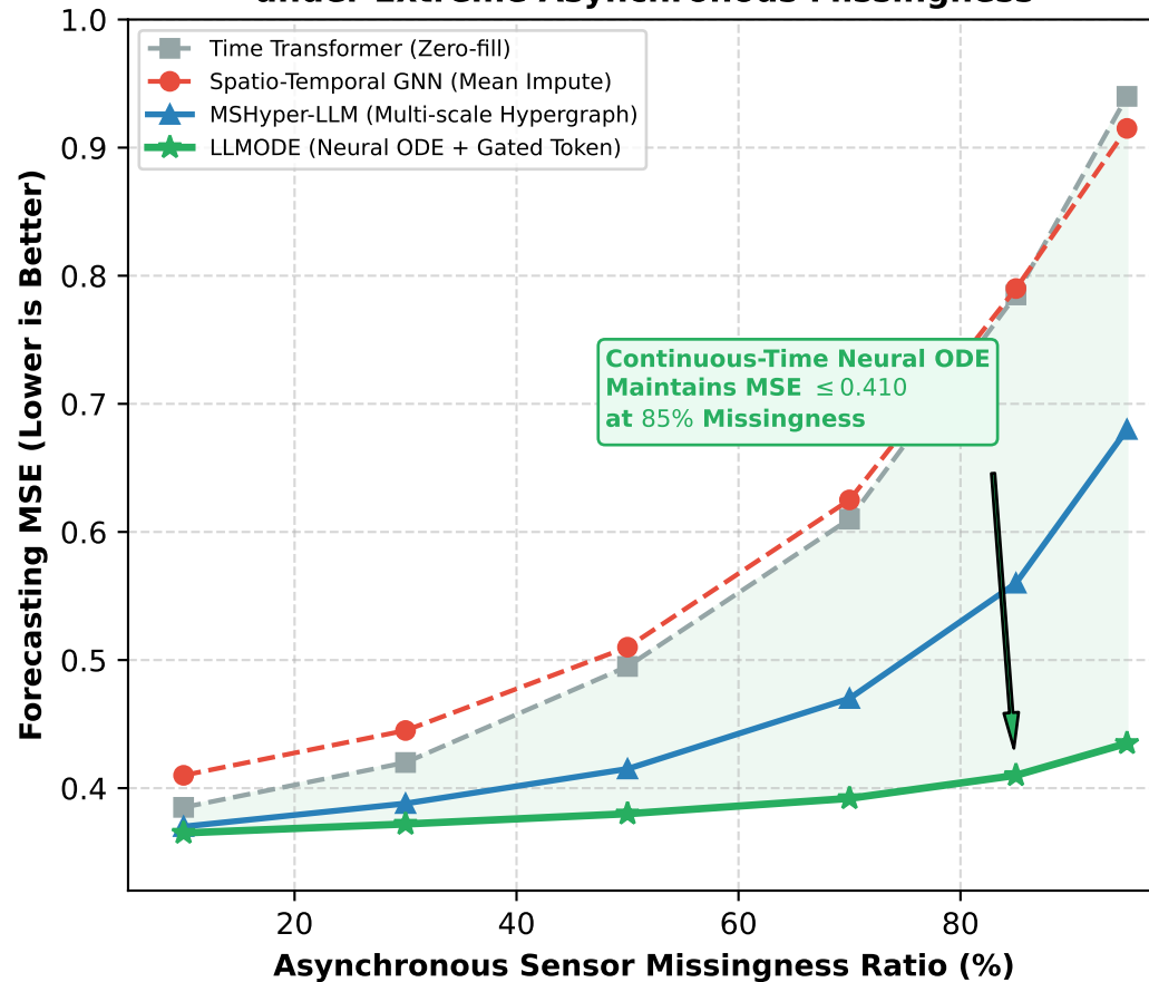
(b) Irregular Spatio-Temporal Forecasting under Extreme Asynchronous Missingness
