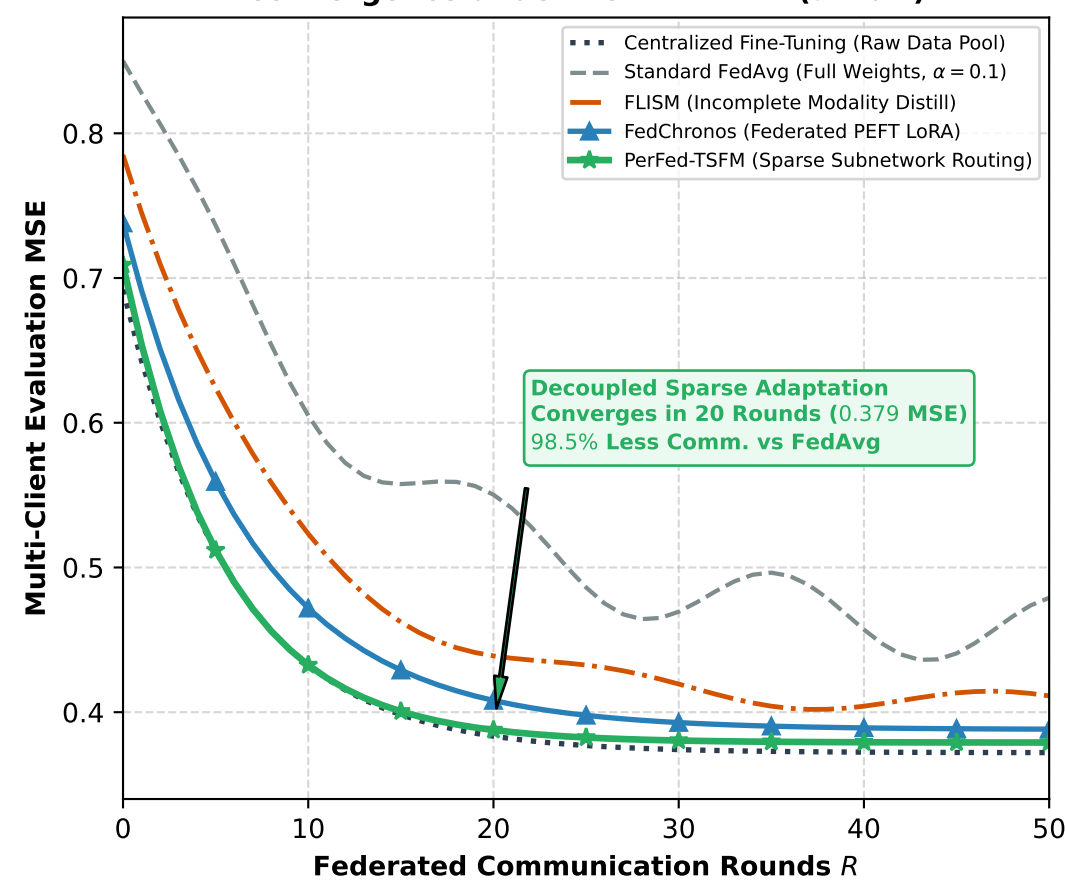
(c) Federated Multimodal TSFM Adaptation Convergence under Non-IID Drift ( \alpha = 0.1 )
