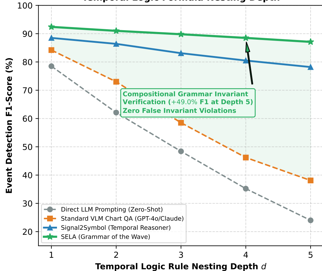
(a) Neuro-Symbolic Logic Verification vs. Temporal Logic Formula Nesting Depth
