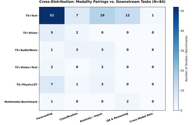
Fig. 12. Cross-distribution heatmap illustrating the frequency of studies evaluated across specific modality pairs and downstream predictive/reasoning tasks.
