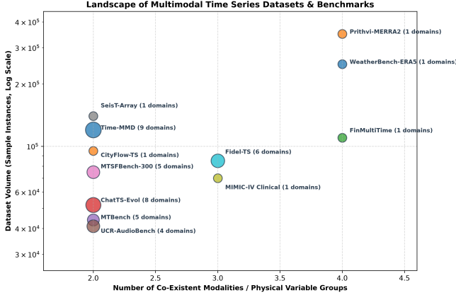
Fig. 13. Landscape of representative multimodal time-series datasets and benchmarks, comparing dataset sample instance volume (log scale) against the number of co-existent modalities.
