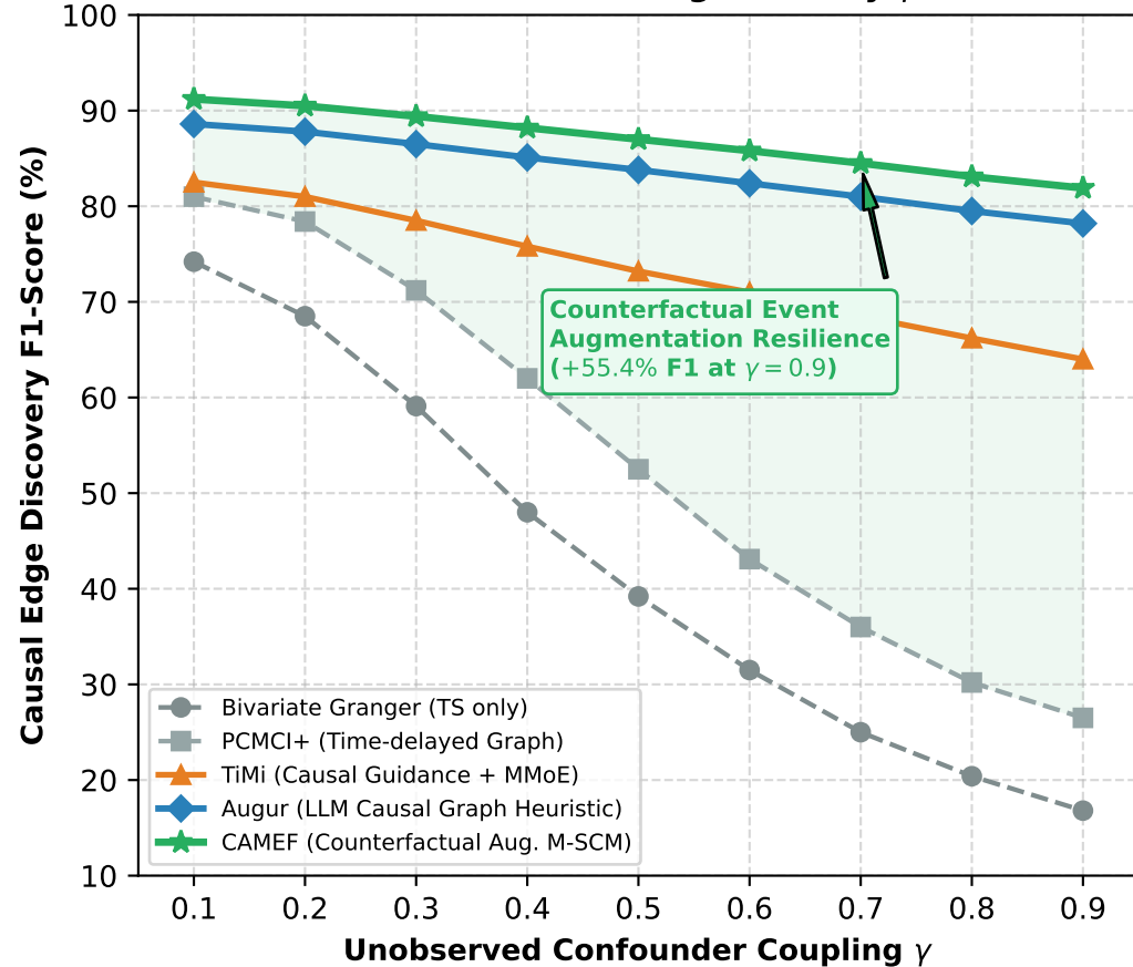
(a) Cross-Modal Causal Graph Discovery under Confounding Intensity \gamma
