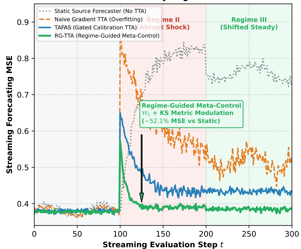
(c) Streaming Test-Time Adaptation under Non-Stationary Regime Transitions
