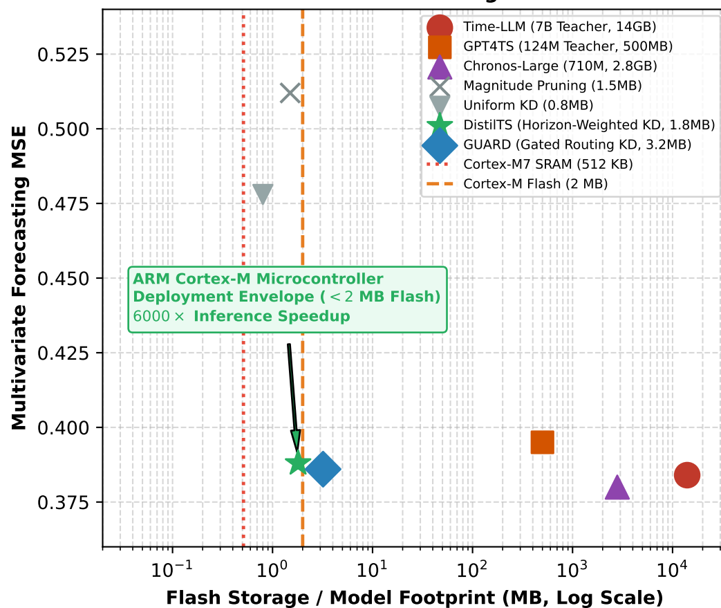
(b) TSFM Distillation Pareto Frontier & Microcontroller Storage Limits
