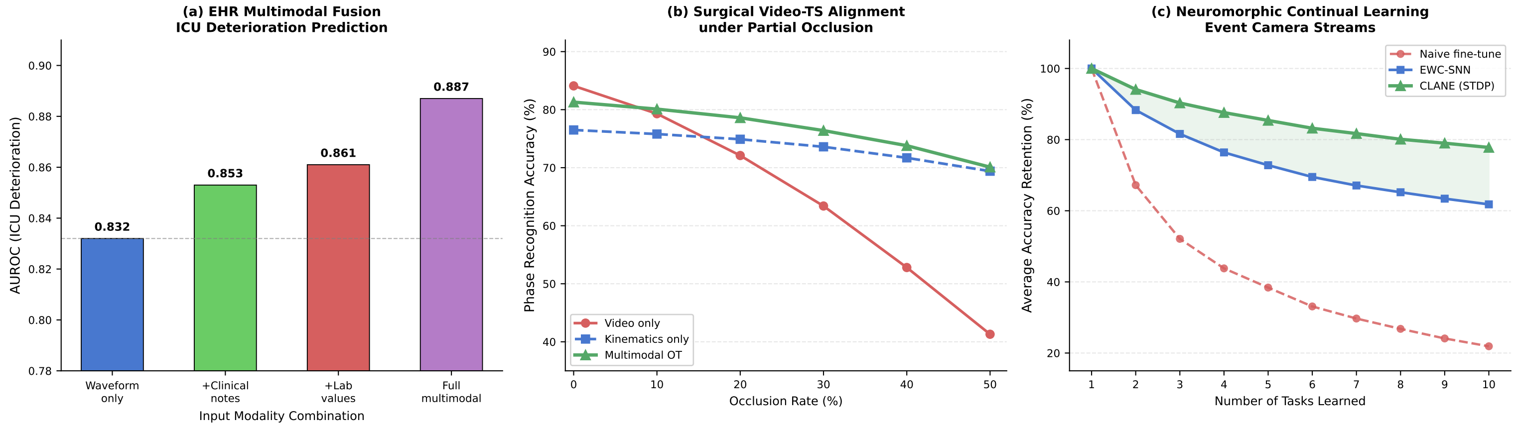
Figure 19: Cross-Modal Clinical EHR, Surgical Robotics Video-TS, and Neuromorphic Continual Learning
