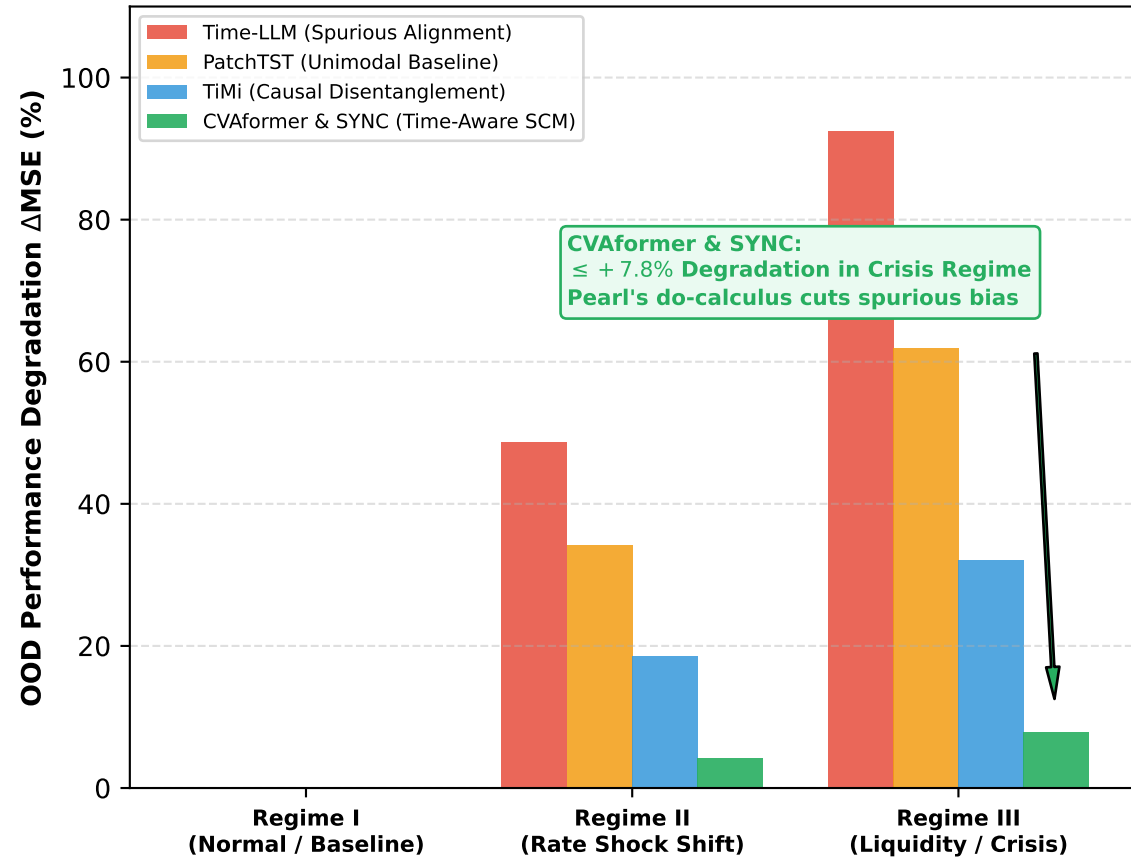
(c) Non-Stationary Regime Generalization: OOD Error Degradation under Shocks
