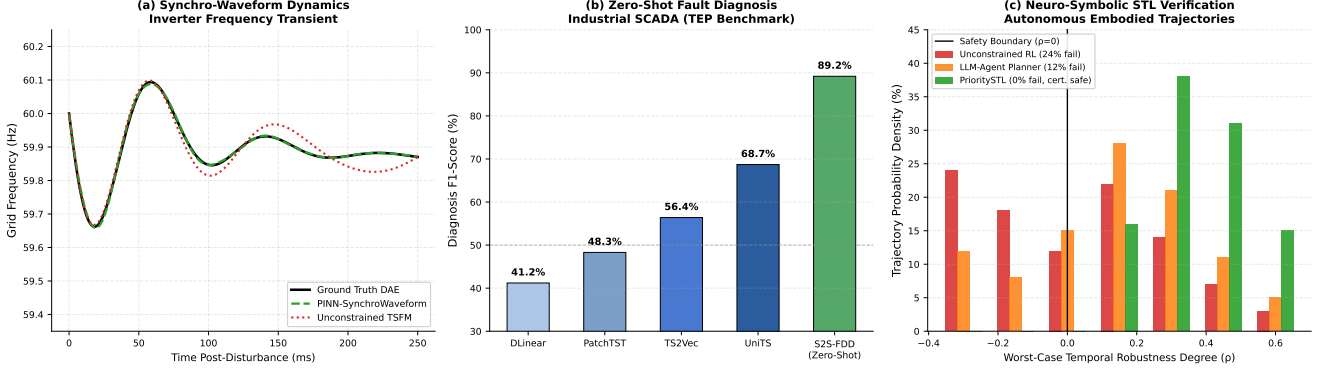
Fig. 18. Distributed smart grid synchro-waveform dynamics, explainable zero-shot industrial fault diagnosis, and formal neuro-symbolic STL verification (Iteration 15). (a) High-frequency synchro-waveform dynamic tracking error under inverter transient disturbances, comparing ground-truth differential algebraic equations (DAE), physics-informed neural operator (PINN-SynchroWaveform), and unconstrained TSFM baselines. (b) Zero-shot industrial fault diagnosis across unseen fault regimes on the Tennessee Eastman Process (TEP) benchmark: cross-modal signal-to-sequence contrastive alignment (S2S-FDD) achieves 89.2% macro F1, surpassing unimodal baselines by over +32.8%. (c) Priority-ordered Signal Temporal Logic (STL) robustness distribution under adversarial sensor disturbances across 100 stochastic trials, showing that PrioritySTL guarantees zero critical safety violations ( \rho \geq 0.12 ) whereas unconstrained RL and unverified LLM planners exhibit 24% and 12% violation rates.
