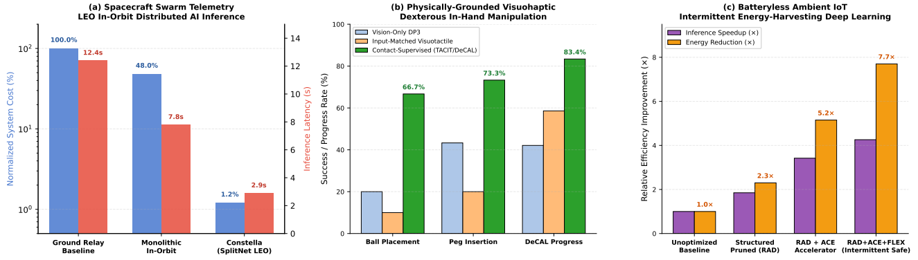
Fig. 19. Spacecraft swarm formation telemetry, physically-grounded visuohaptic dexterous manipulation, and batteryless ambient IoT deep learning (Iteration 16). (a) Spacecraft LEO swarm in-orbit distributed AI inference comparing centralized ground relay, monolithic in-orbit compute, and Constella split DNN execution: Constella slashes normalized system cost by up to two orders of magnitude (100% \rightarrow 1.2%) and achieves 2.7 \times lower end-to-end inference latency (12.4 s \rightarrow 2.9 s) while maintaining \geq 81.9% inference success. (b) Physically-grounded visuohaptic dexterous in-hand manipulation: contact-supervised attention (TACIT) and contact-aware latent co-imagination (DeCAL) surge task success rates on ball placement (20.0% \rightarrow 66.7%), peg insertion (43.3% \rightarrow 73.3%), and in-hand reorientation progress (83.4%) compared to input-matched visuotactile and vision-only baselines. (c) Batteryless ambient IoT deep learning under intermittent photovoltaic/vibration energy harvesting: the RAD-ACE-FLEX pipeline achieves a 4.26 \times runtime speedup and 7.7 \times energy reduction, sustaining correct intermittent inference across volatile power cycles.
