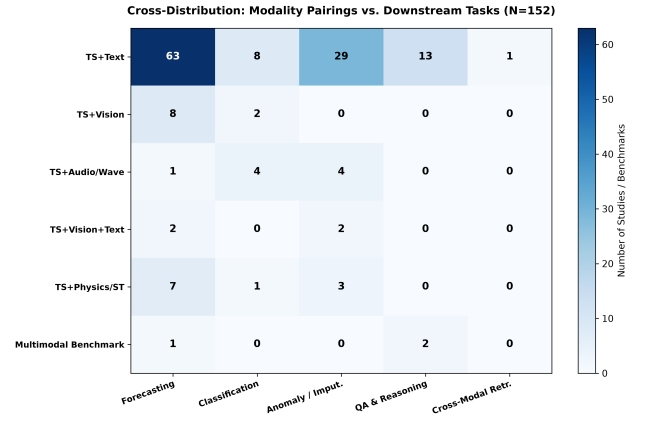
Fig. 20. Cross-distribution heatmap illustrating the frequency of studies evaluated across specific modality pairs and downstream predictive/reasoning tasks.
