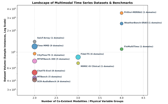
Fig. 21. Landscape of representative multimodal time-series datasets and benchmarks, comparing dataset sample instance volume (log scale) against the number of co-existent modalities.
