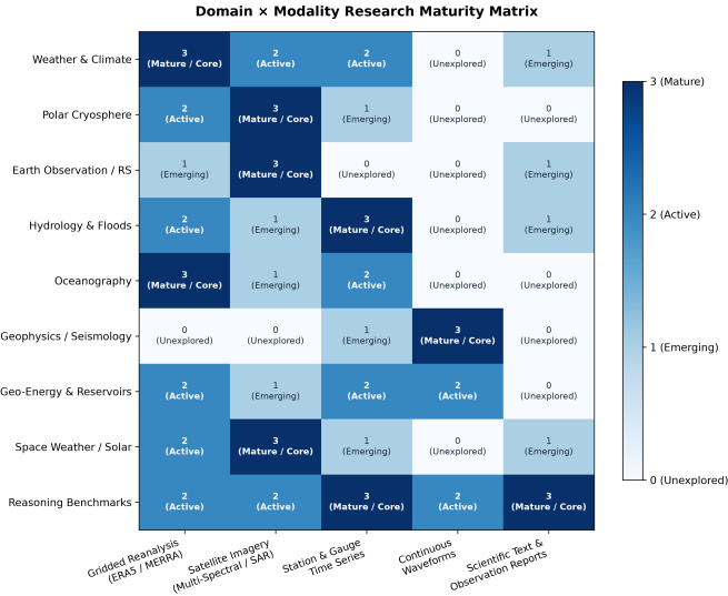
Fig. 2. Domain × Modality Research Maturity Matrix, highlighting established core areas and emerging multimodal frontiers across N = 95 verified studies.
