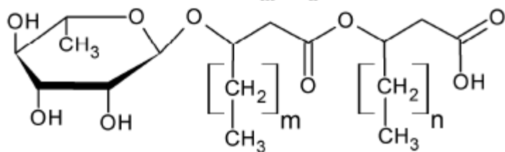
Di-rhamnolipids
