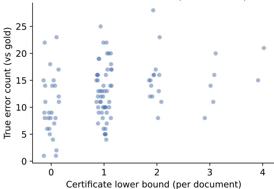
Certificate bound vs. true errors — DeepSeek-V3 (Spearman \rho=0.25 )
