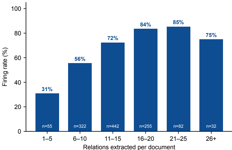
Firing rises with output volume (per document, N=1188)
