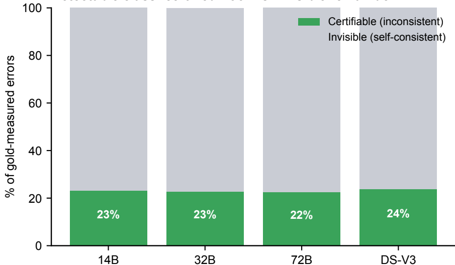
Detectable class: certified floor vs invisible remainder
