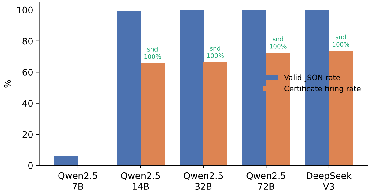
Certificate across the model-capability gradient (soundness=100% throughout)
