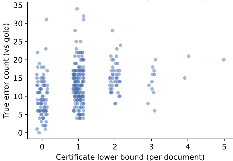
Certificate bound vs. true errors — DeepSeek-V3 (Spearman rho=0.28)
