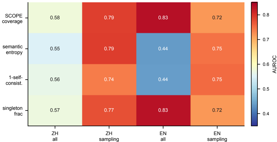
Triage AUROC across datasets, targets, and signals
