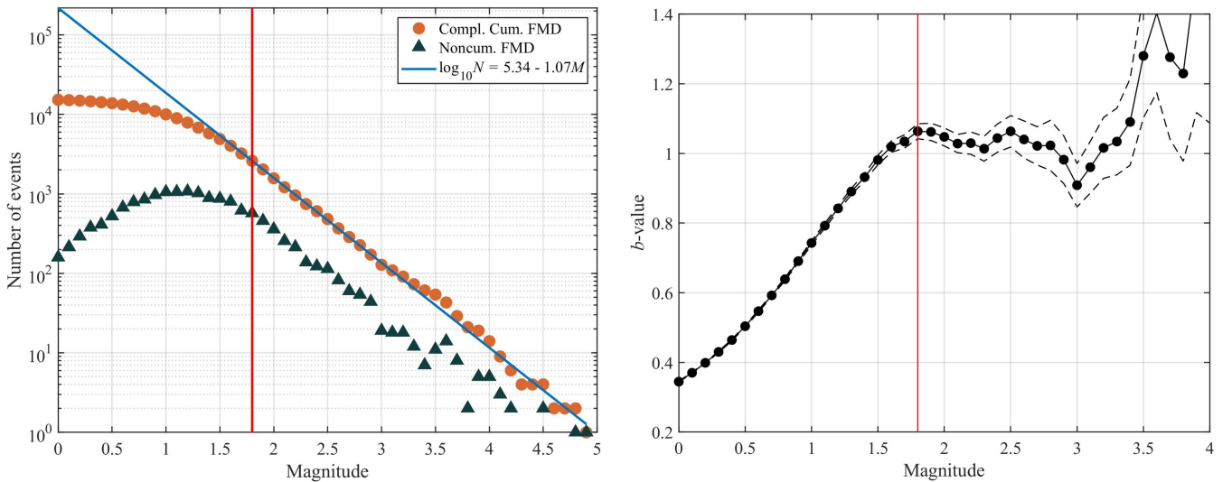
Figure 5. (left) Complementary cumulative and density frequency-magnitude distribution of seismicity from the previous half year in the CSES, alongside the Gutenberg-Richter (GR) law fitted using earthquakes with M \geq M_c , where M_c is derived for the previous half year (red vertical line); (right) Variation of the b -value of the GR law with M_c , with the thin dashed lines indicating the \pm 1\sigma standard deviation boundaries.
